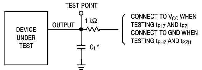
Figure 7. Test Circuit
